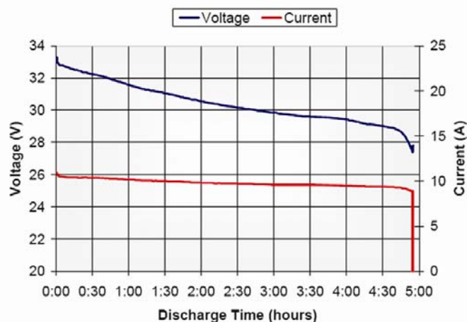
Figure 3 Voltage and Current during a battery discharge at 10,000 psi
